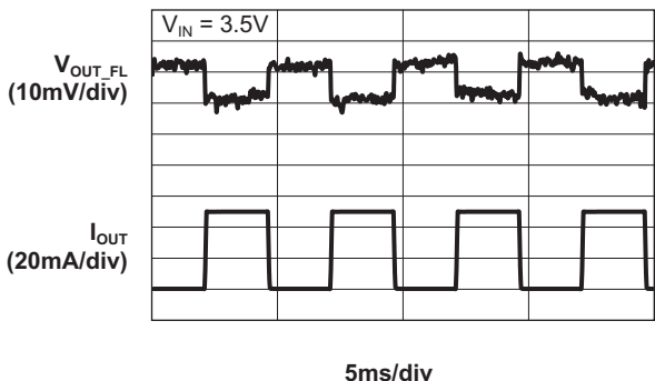
Load Response vs. Time (50mA Load)
