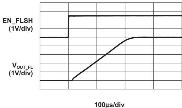
Start-Up Time (50mA Load)
